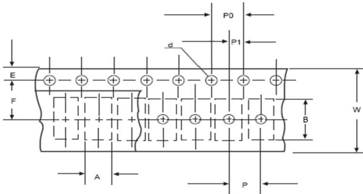
Fig 3. Carrier tape dimensions
