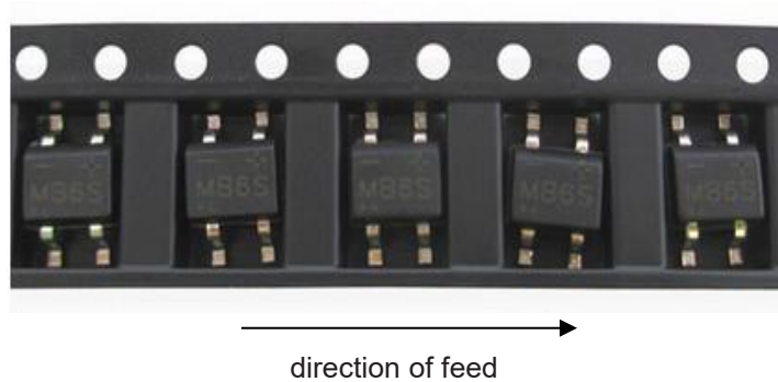
Fig 2. Product orientation in carrier tape
